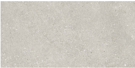
Basalt
